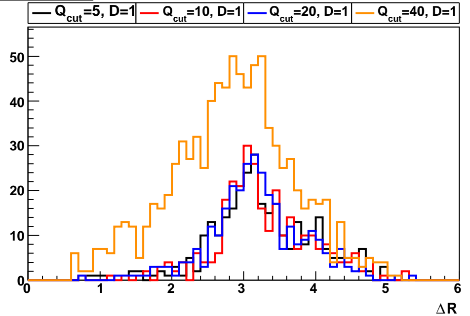
largest jet \Delta R
