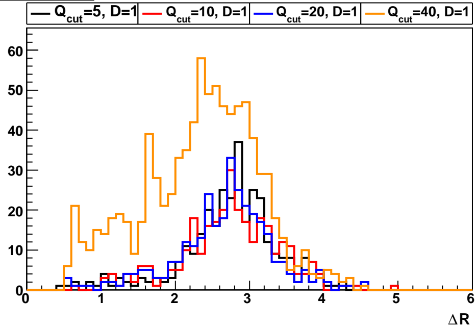
middle jet \Delta R
