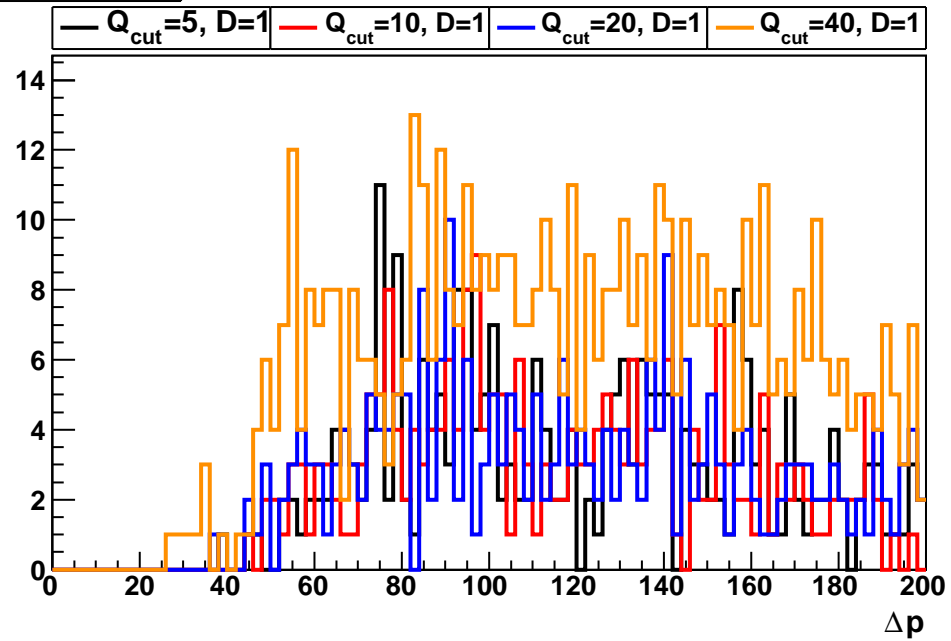
largest jet \Delta p
