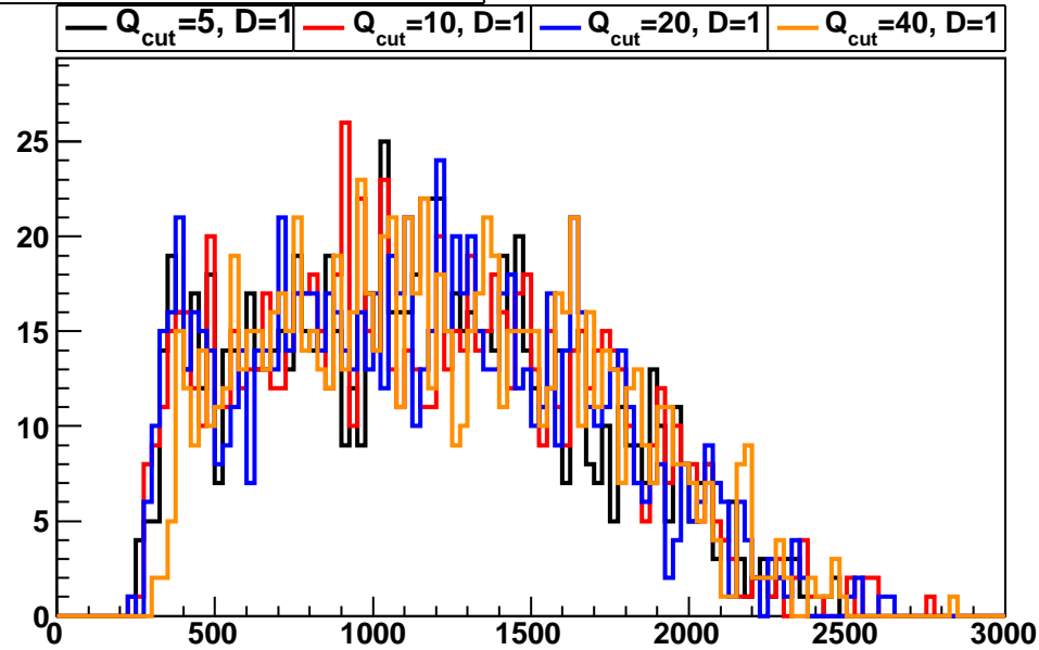
total number of truth particles
