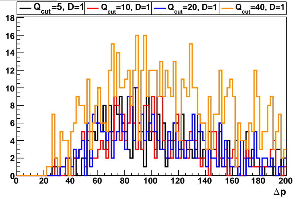
middle jet \Delta p
