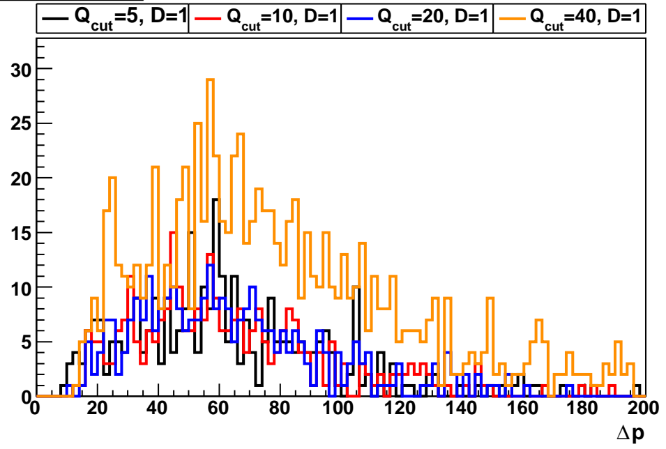
smallest jet \Delta p
