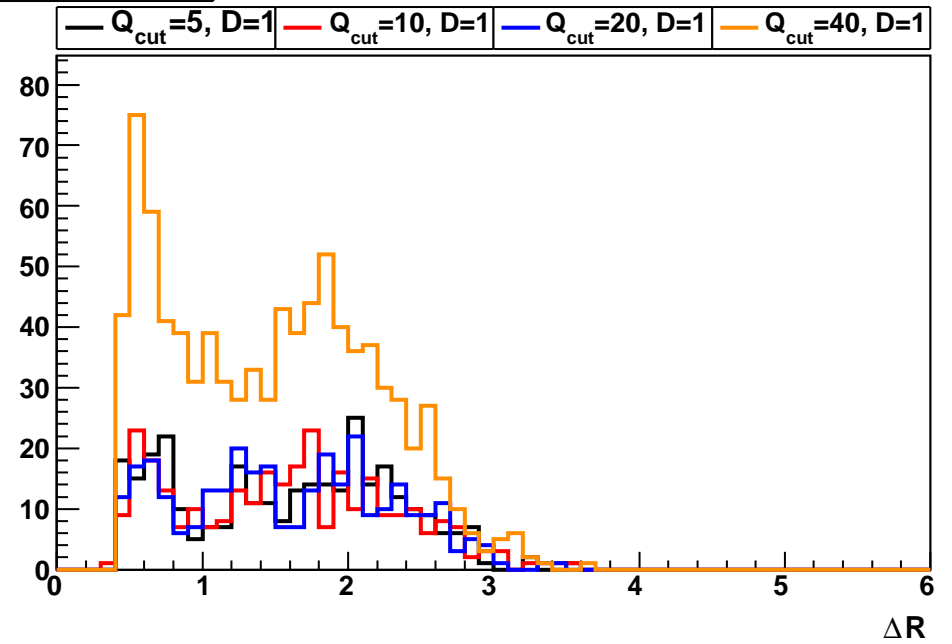
smallest jet \Delta R
