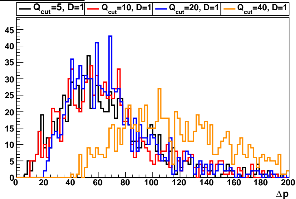
smallest parton \Delta p
