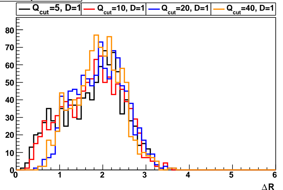
smallest parton \Delta R
