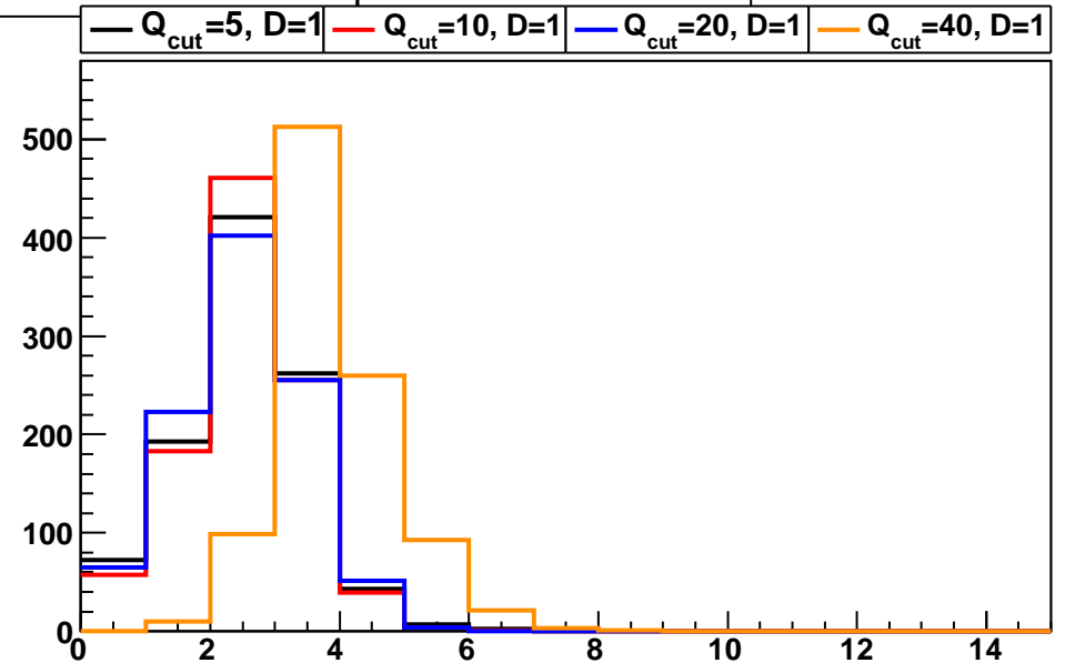
number of jets with p_{\text{T}} \geq 20 \text{ GeV}/c and |\eta| < 2.5
