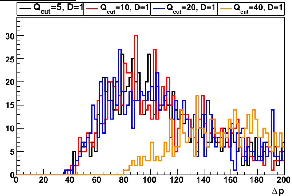
middle parton \Delta p
