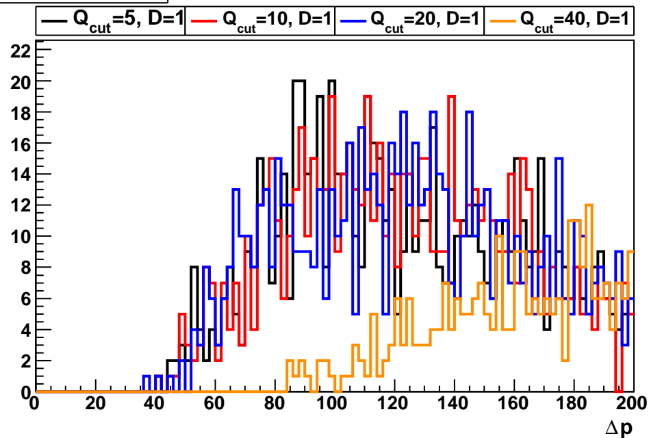
largest parton \Delta p
