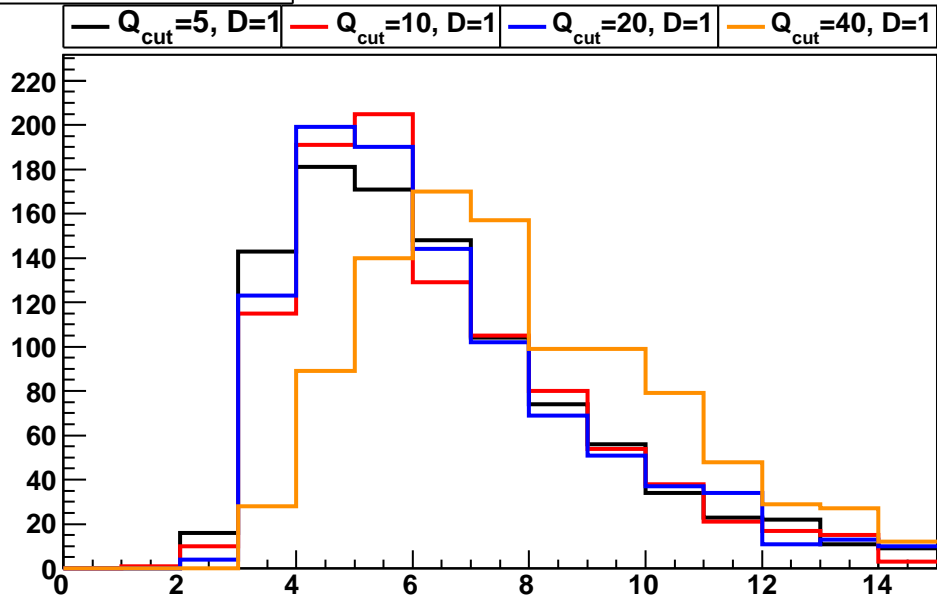
total number of jets
