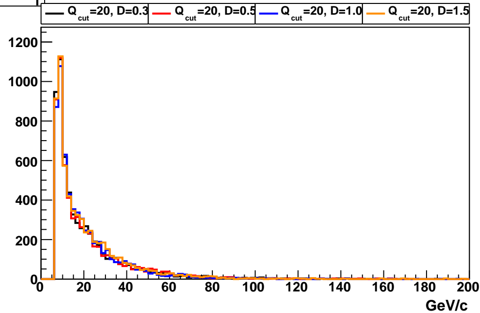
jet p_T
