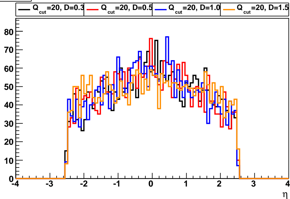
parton \eta
