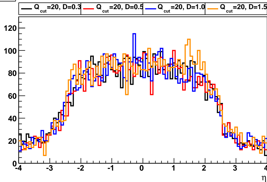
jet \eta
