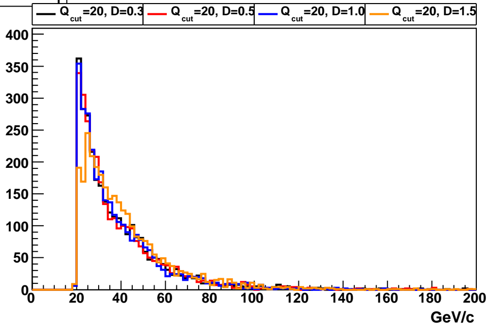
parton p_T
